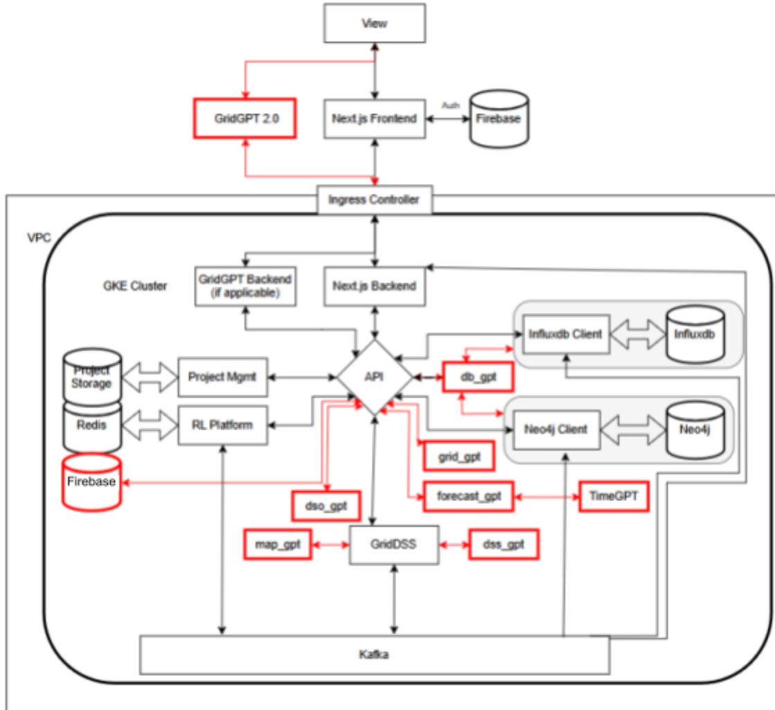
FIGURE 5: GridGPT 2.0 + GridAI Design
